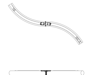
18. Code 227010A 45° CURVE RIGHT - 45° CURVE RIGHT JOINT
