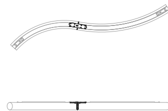
08. Code 2257010A 60° CURVE - 45° CURVE S JOINT
