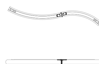
16. Code 2258010A 45° CURVE - 60° CURVE S JOINT
